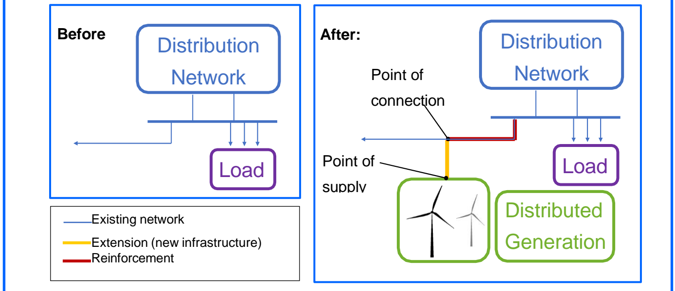
Figure 16: Illustration showing extension and reinforcement of the network.
