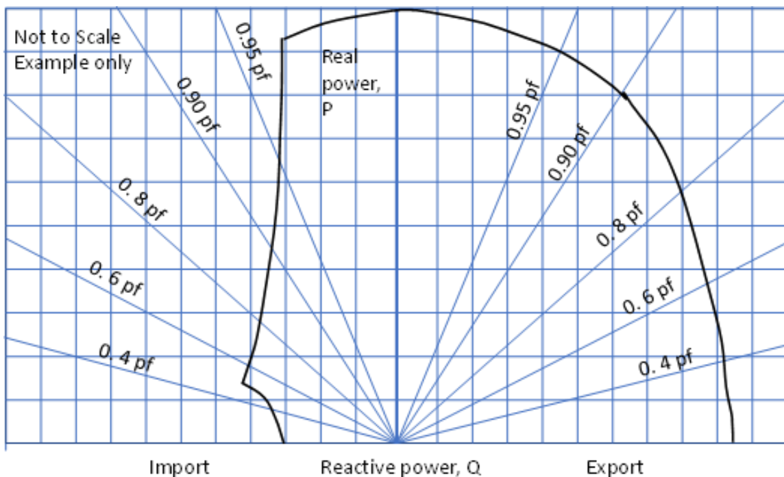
Figure 13: Typical chart provided by the manufacturer showing the active power capability of the Power Generating Facility
